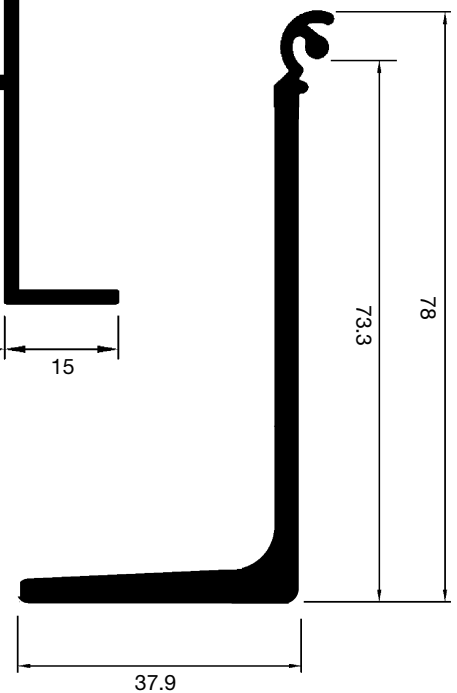
L Bar to Suit 50mm & 87mm Reversible Lath Section 25575
