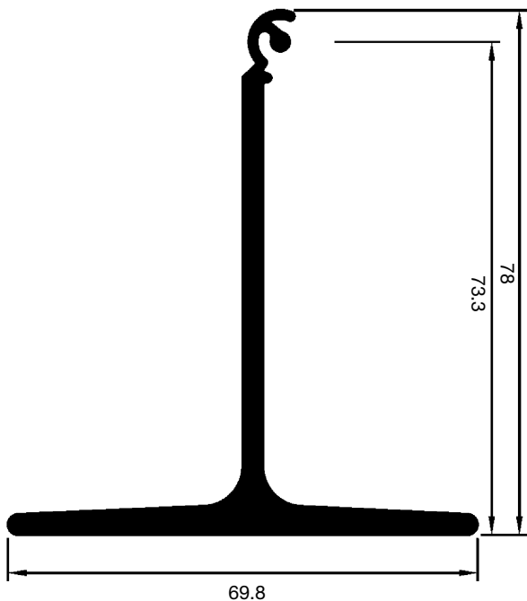
T Bar to Suit 50mm & 87mm Reversible Lath Section 18573
