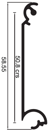
50mm Reversible Roll Shutter Lath (2") Section 18499
