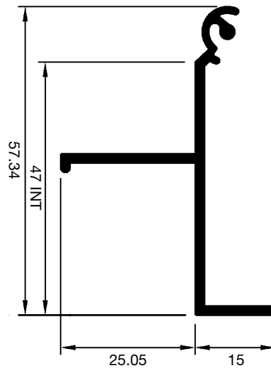
50mm & 87mm Reversible Lath Section 20850
