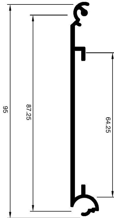
87mm Reversible Roll Shutter Lath (3½") Section 20849
