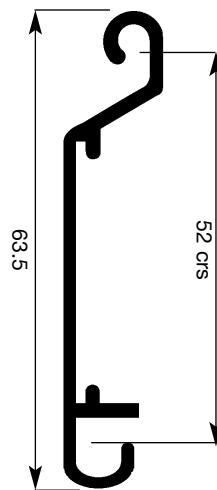
63.5mm Reversible Roll Shutter Lath (2") Section 29596
