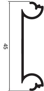
Adaptor Used to mate Laths with Tubes & Links Section 26034
